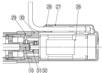
In-line motor type: LEY 16 25 32 40 D
