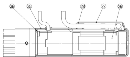
In-line motor type: With lock/motor cover
