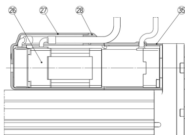
In-line motor type: LEY 16 25 32 D 40
