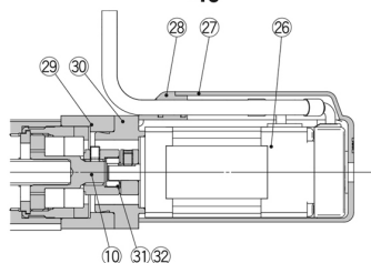
In-line motor type: LEY 16 25 32 D 40
