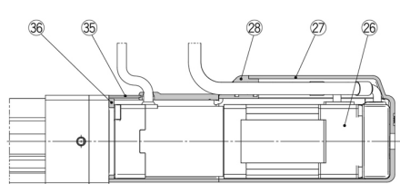
In-line motor type: With lock/motor cover
