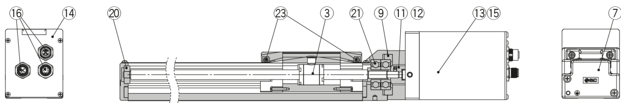
In-line motor
