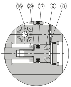
Piston rod B-side piston
