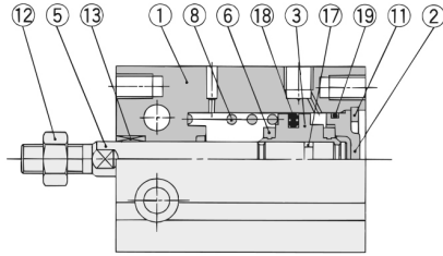
ø16 to ø32 Single acting, Spring return
